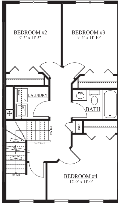
SECOND FLOOR OPTION B
