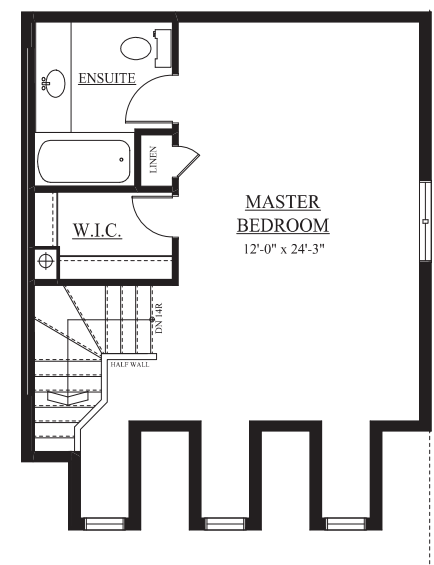
THIRD FLOOR OPTION B
